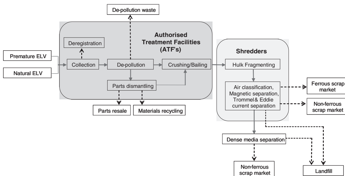
Fig. 1 The flow of the vehicle through EoL operations
